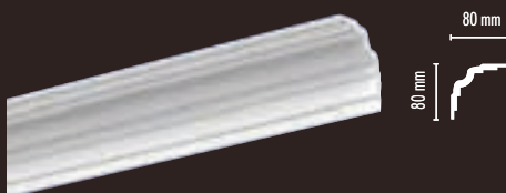
WT25 80 mm x 80 mm • 3 1/8" x 3 1/8"
