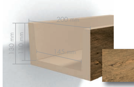
Beam 13-20 DARK-BROWN Beam 13-20 LIGHT-BROWN Length 3m, 4m
