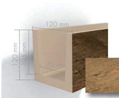
Beam 12-12 DARK-BROWN Beam 12-12 LIGHT-BROWN Length 2m, 3m, 4m
