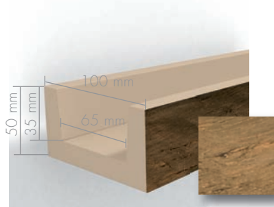
Beam 05-10 DARK-BROWN Beam 05-10 LIGHT-BROWN Length 2m, 3m, 4m
